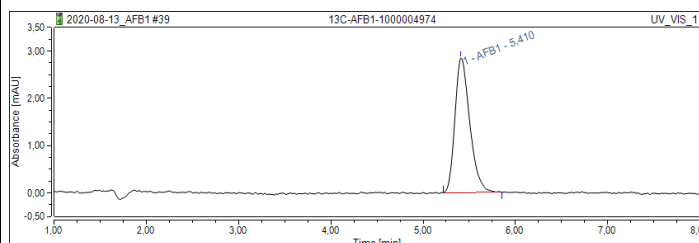
Figure 1: HPLC-UV chromatogram of U-[ 13 C 17 ]-Aflatoxin B1
